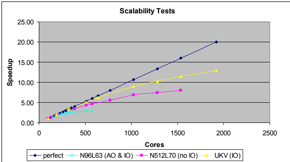
Figure 2: Performance vs compute resource
